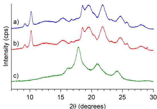
Figure 2. Powder XRD profiles of (a) poly( S -propylene succinate), (b) poly( R -propylene succinate), and (c) stereocomplexed poly(propylene succinate).
